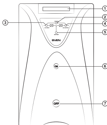
Fig. 1. Front panel
