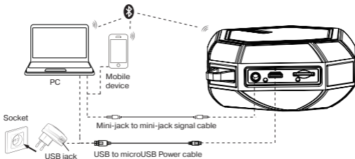
Fig. 2. Connection diagram
