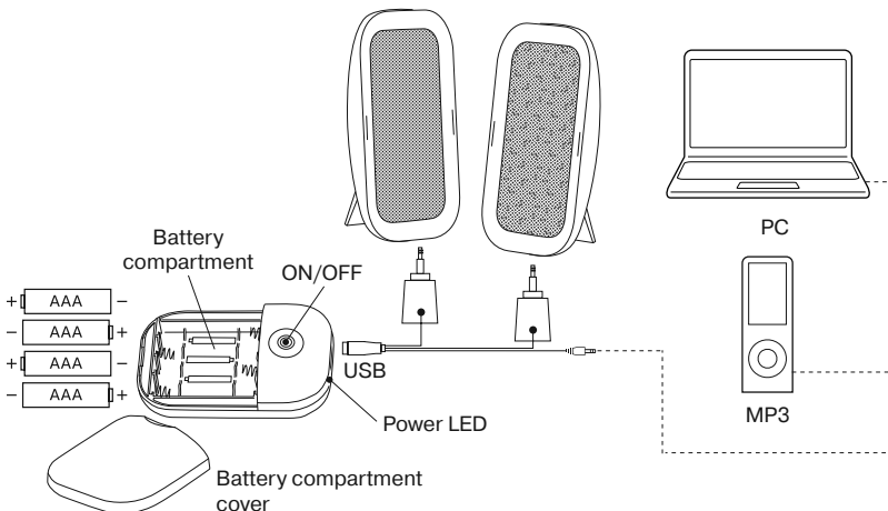
Fig. 1. Connection diagram
