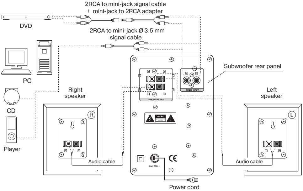
Fig. 3. Connection diagram
