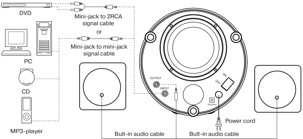
Fig. 3. Connection diagram
