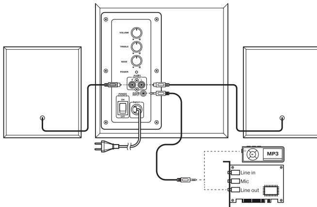
Fig. 2. Connection diagram
