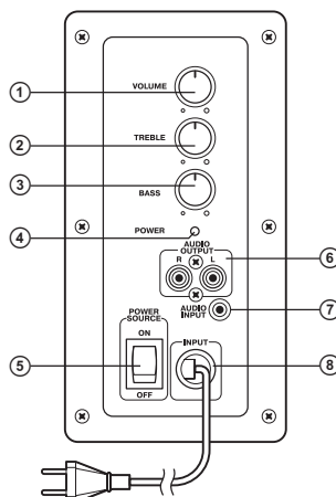
Fig. 1. Control panel
