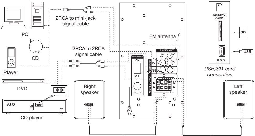
Fig. 5. Connection diagram
