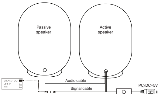
Fig. 2. Connection diagram
