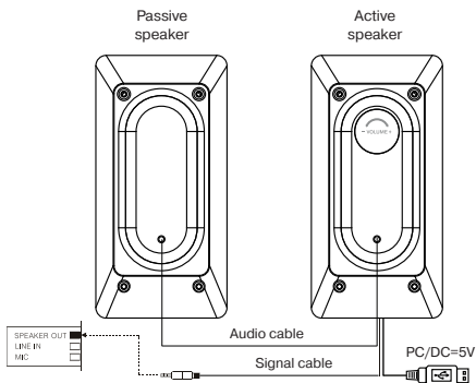
Fig. 2. Connection diagram
