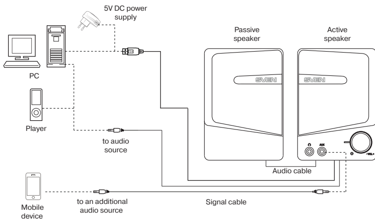
Fig. 2. Connection diagram
