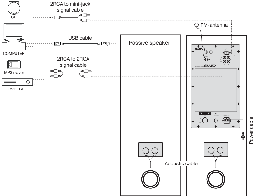
Fig. 5. Connection diagram
