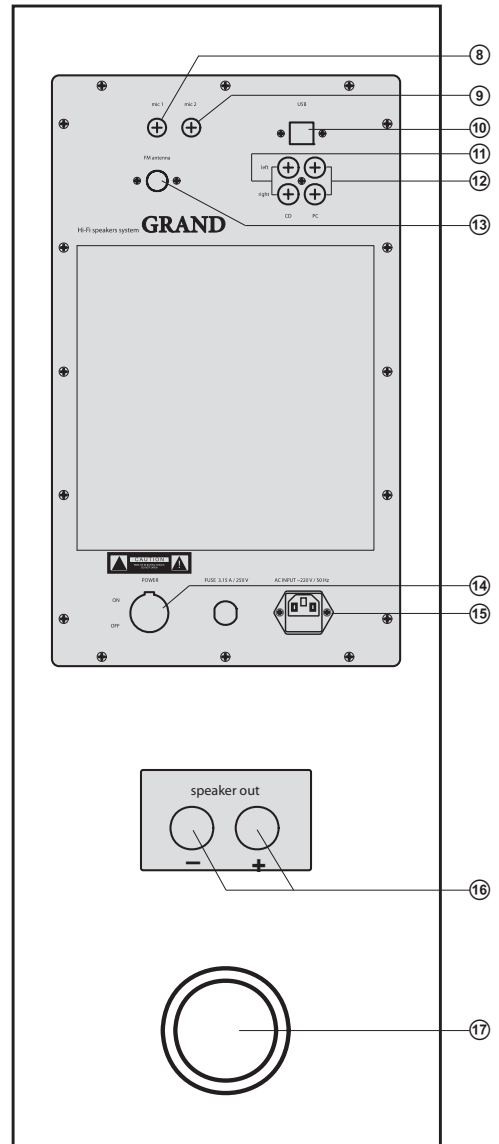
Fig. 3. Active speaker rear panel
