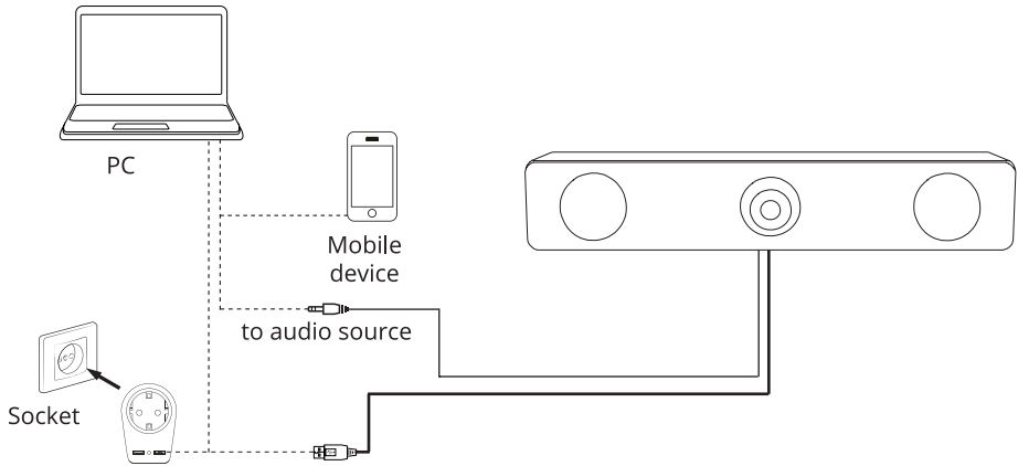
Fig. 2. Connection diagram
