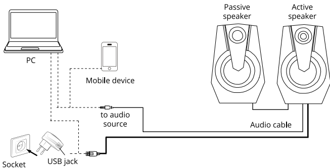
Fig. 2. Connection diagram
