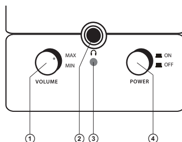
Fig. 1. Control panel
