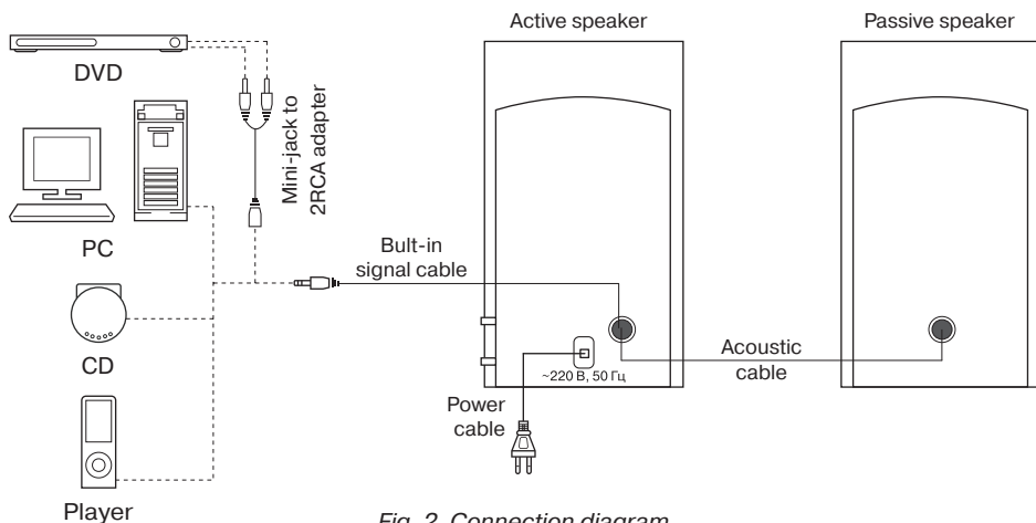
Fig. 2. Connection diagram
