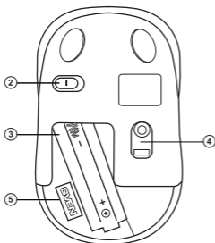
Fig. 2. Bottom view
