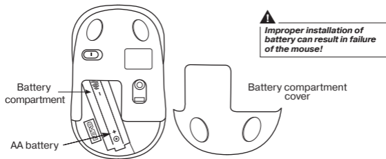
Fig. 4. Battery installation
