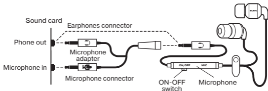
Fig. 1. Connection diagram
