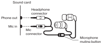
Fig. 1. Connection diagram
