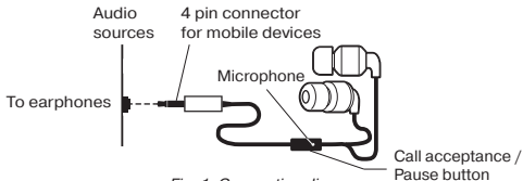
Fig. 1. Connection diagram
