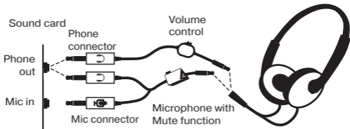
Fig. 1. Connection diagram
