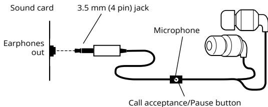
Fig. 1. Connection diagram
