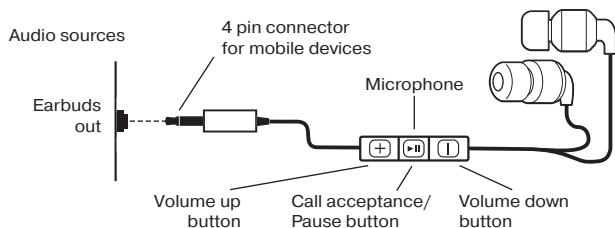
Fig. 1. Connection diagram
