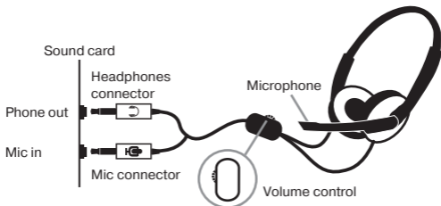
Fig. 1. Connection diagram
