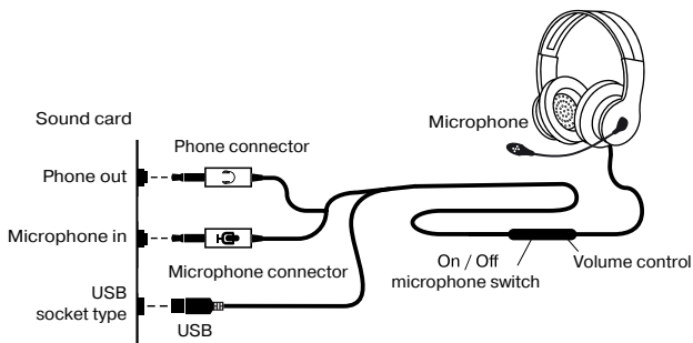
Fig. 1. Connection diagram
