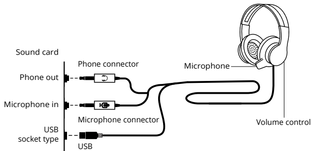
Fig. 1. Connection diagram
