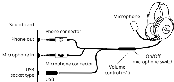
Fig. 1. Connection diagram
