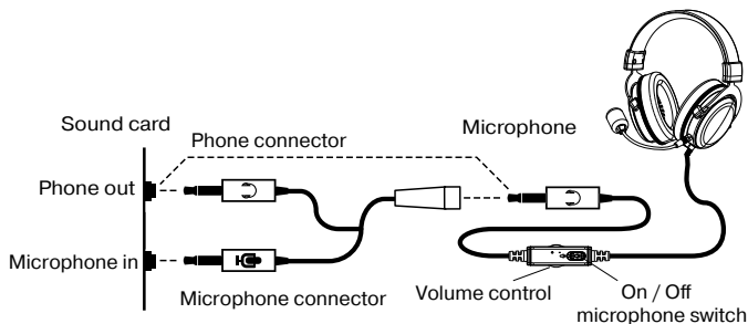
Fig. 2. Connection diagram
