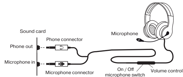
Fig. 1. Connection diagram
