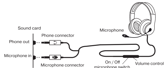
Fig. 1. Connection diagram
