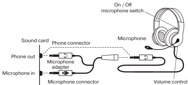
Fig. 1. Connection diagram
