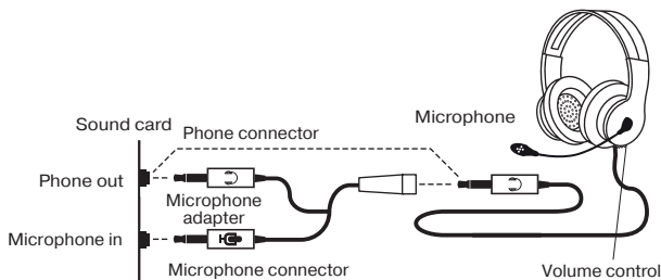
Fig. 1. Connection diagram
