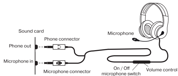
Fig. 1. Connection diagram
