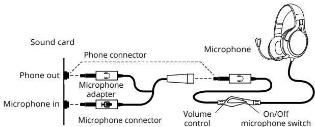
Fig. 2. Connection diagram
