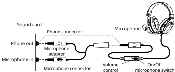
Fig. 2. Connection diagram
