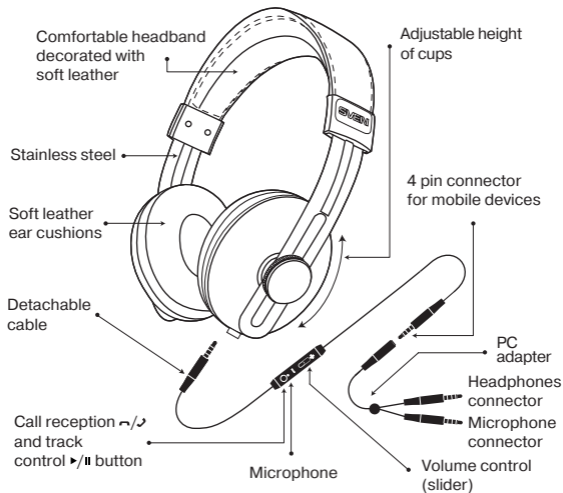
Fig. 1. Connection diagram
