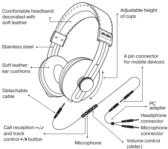
Fig. 1. Connection diagram
