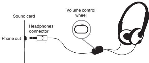
Fig. 1. Connection diagram
