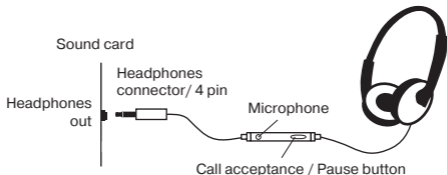
Fig. 1. Connection diagram
