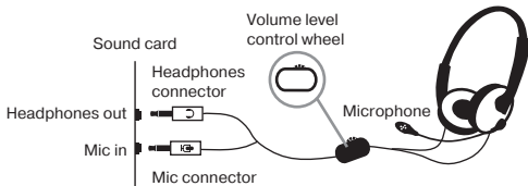
Fig. 1. Connection diagram
