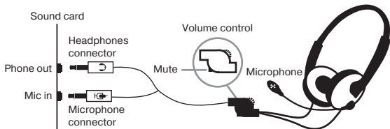
Fig. 1. Connection diagram
