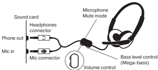
Fig. 1. Connection diagram
