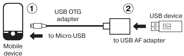
Connection diagram
