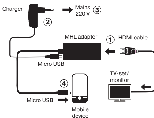
Connection diagram
